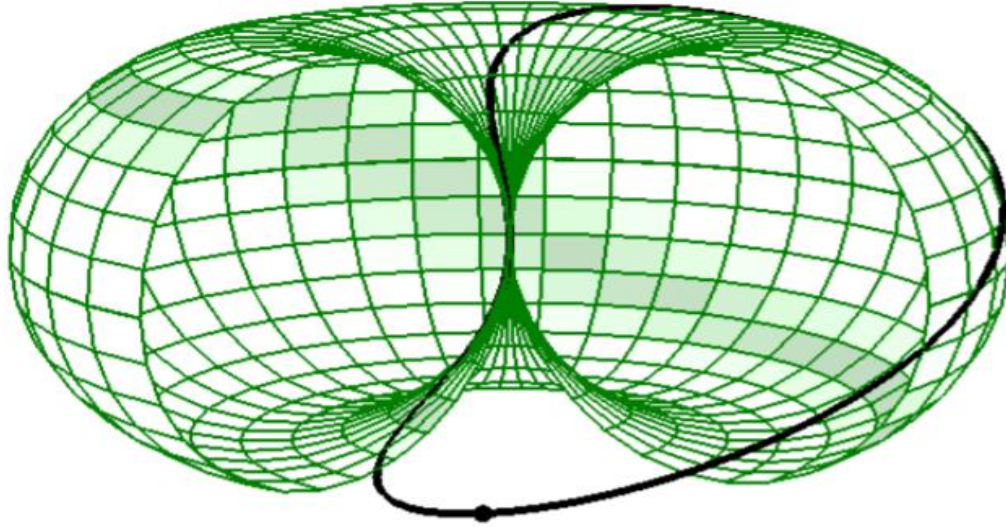
Fig. 1. The univon model composed of a superluminal primordial information quantum (spring). The mathematical horn torus surface on which the spring travels is cut away to show the interior. The black closed curve on the surface of the horn torus is the trajectory of the univon's spring (indicated by the black dot.)
