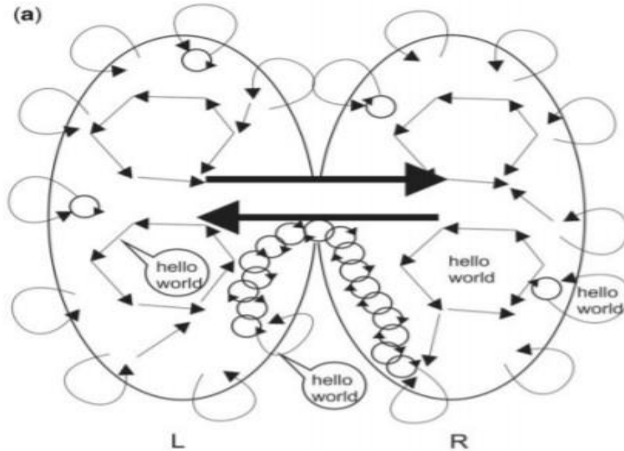
Figure 5. Adopted from Kozłowska and Kozłowski. The formula represents the elementary value of quantum energy for brain and Schumann waves.
