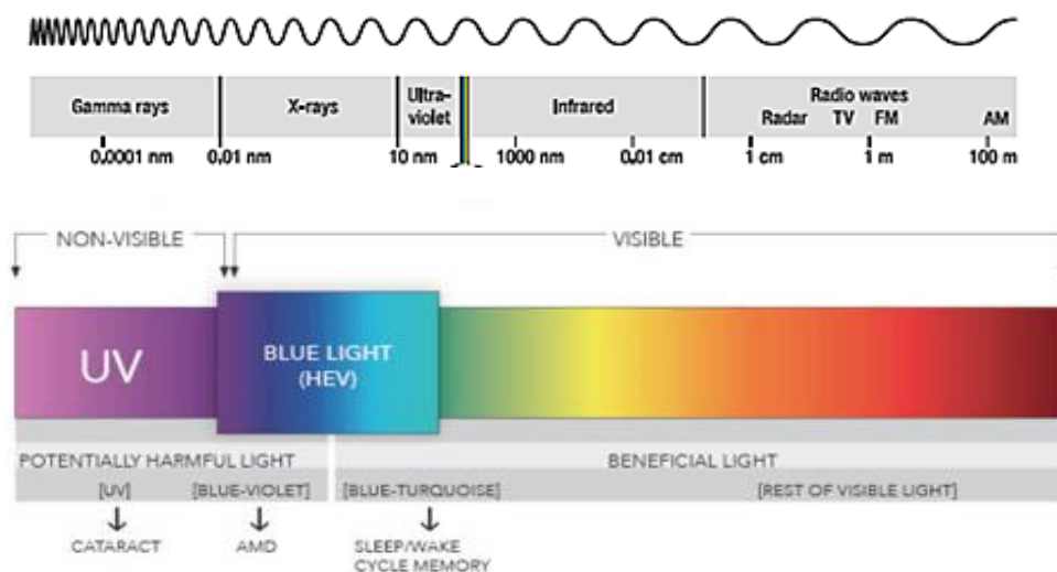
Fig. 1. Part of the visible light spectrum, blue light is the high energy spectrum just beyond the UV light. Over exposure to the blue light may lead to harmful effects.
